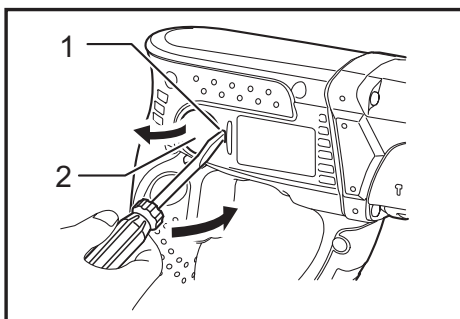
► 1. Recessed part 2. Holder cap cover
